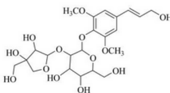
Figure 24 Syringenine 4-O-apiosyl-glucoside
