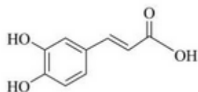
Figure 19 Acide Caféique
