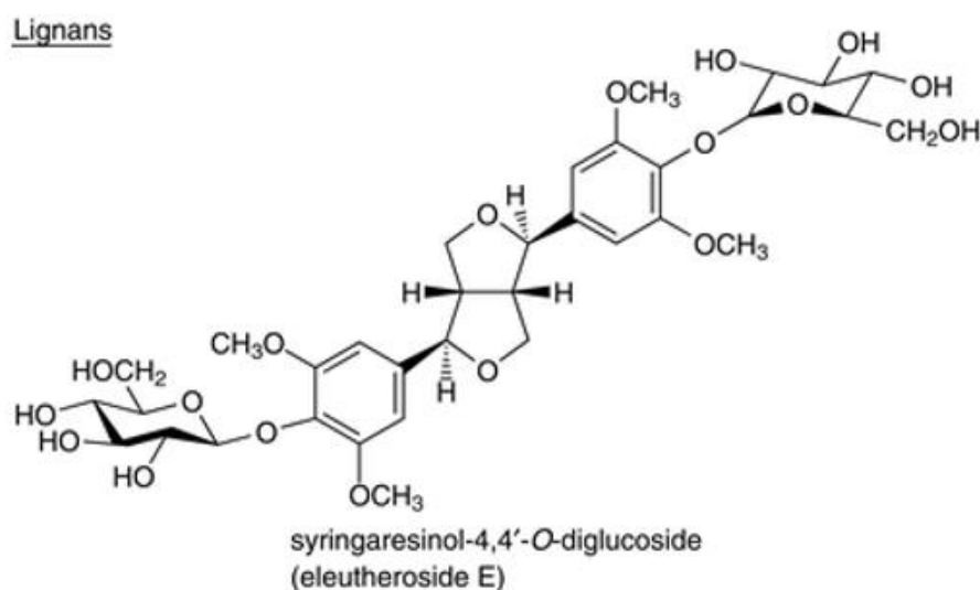
Figure 17 Eleuthéroside E (32)
