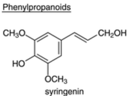
Figure 18 Syringine (32)
