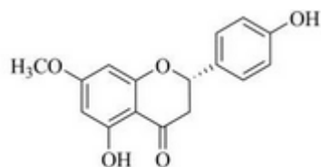
Figure 21 Sakuranetine
