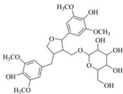
Figure 25 Alangilignoside C
